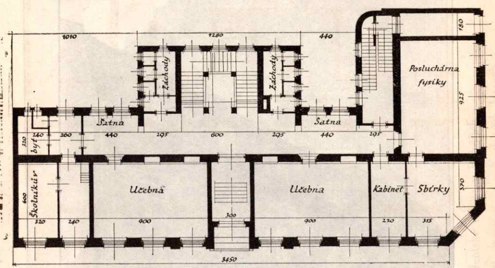
Prizemi
